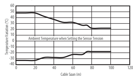
Figure 7 - Thermal Expansion Chart
