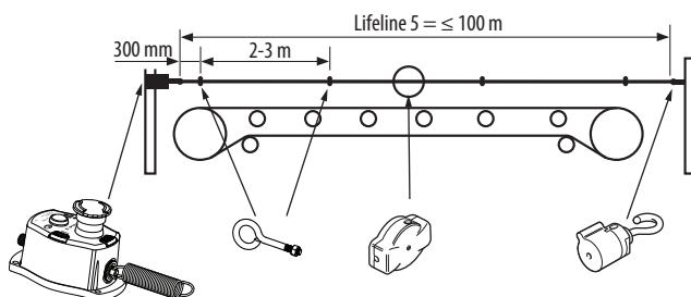
Figure 5 - Typical Mounting Example with One Switch
