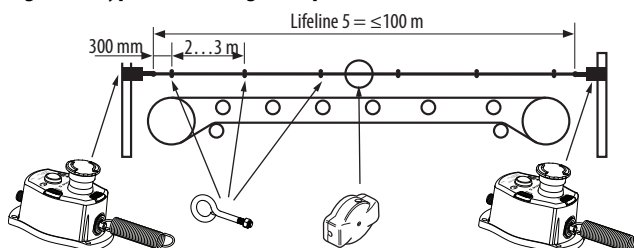
Figure 6 - Typical Mounting Example with Two Switches
