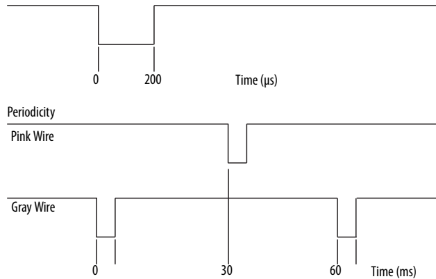
Figure 3 - Individual Pulses
